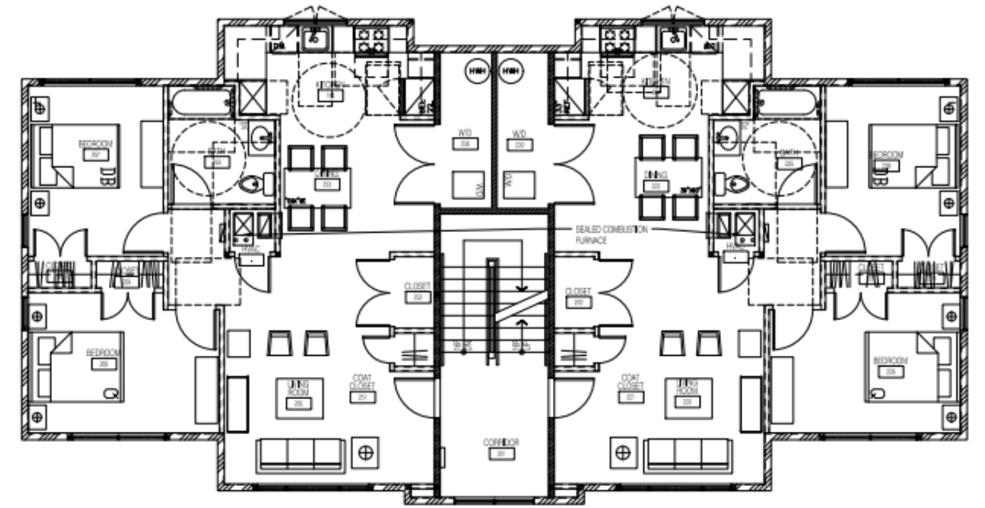
FLEMINGTON AFFORDABLE HOUSING SECOND FLOOR PLAN OPTION 2.1 - 3/1/24
