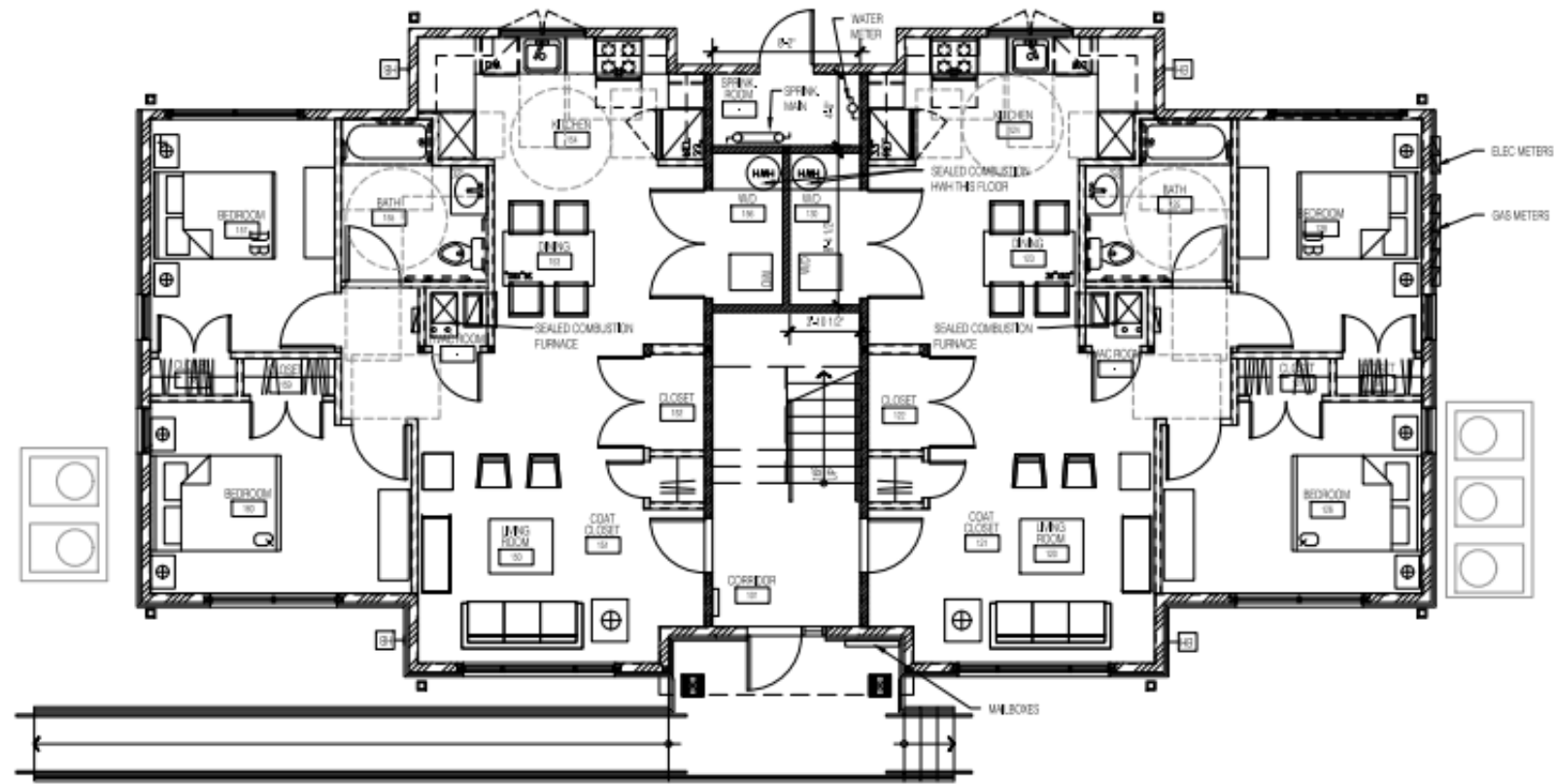
FLEMINGTON AFFORDABLE HOUSING FIRST FLOOR PLAN OPTION 2.1 - 3/1/24
