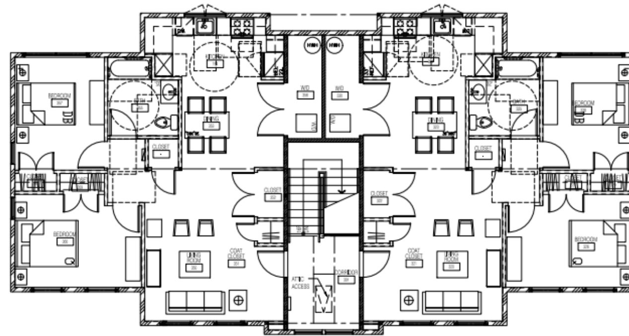
FLEMINGTON AFFORDABLE HOUSING THIRD FLOOR PLAN OPTION 2.1 - 3/1/24
